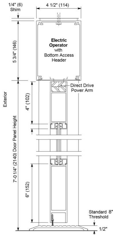
Vertical Section '1'
