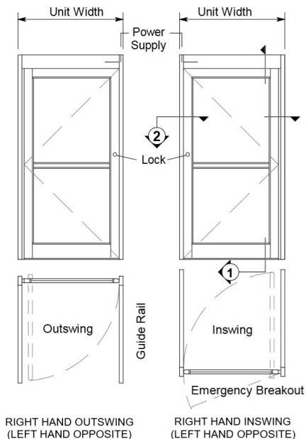
Exterior Elevations and Floor Plans
